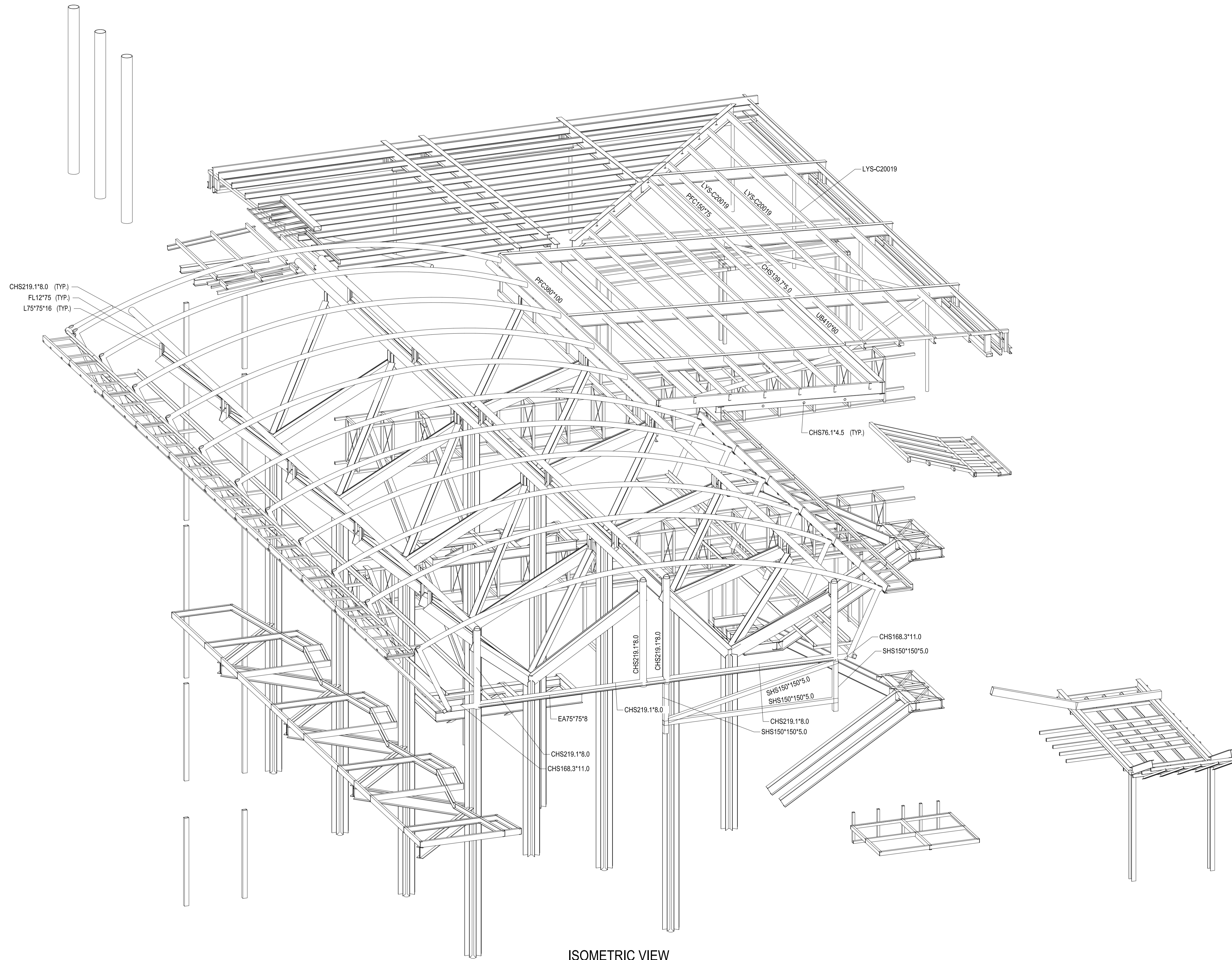
ISOMETRIC VIEW
